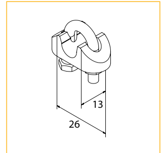
19. Rope Clamp (set of 3)
